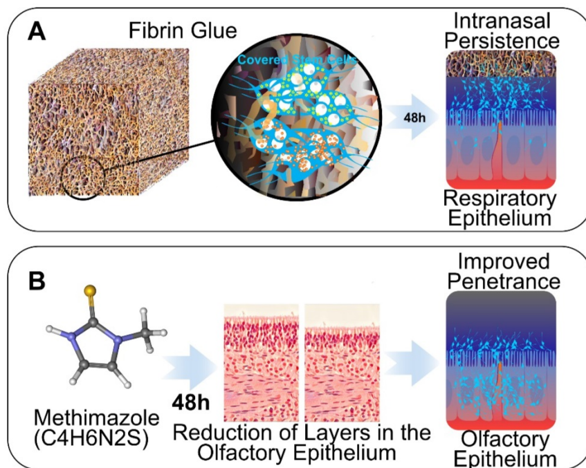
Figure 1. Schematic of strategies to enhance IN delivery of therapeutic neural stem cells (NSCs) to glioblastoma. A , The biocompatible 3 dimensional structure of fibrin glue is utilized to seal NSCs in a nasal cavity to delay clearance and enhance persistence. B , The effect of MT on the disruption of the olfactory epithelium barrier is utilized to improve the brain entry of NSCs through olfactory route.
