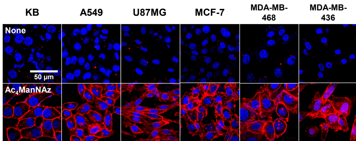
Figure S1. Introduction of unnatural sialic acids with azide groups on the surface of various cells
