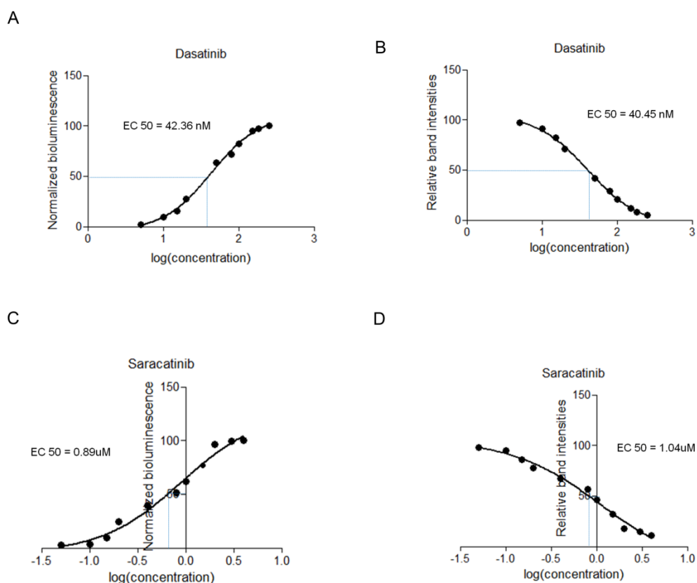
Figure S1. EC 50 values of Src inhibitors estimated by the BSR reporter and Western blot. (A) EC 50 of dasatinib for Src activity inhibition calculated with BSR reporter, by setting the normalized luciferase activity of the vehicle control as 0% and the maximum increased activity of drug treatments as 100%. (B) EC 50 of dasatinib for Src activity inhibition estimated by the relative band intensities (% of vehicle control) of Western blot using phospho-Src antibodies. (C) EC 50 of saracatinib for Src activity inhibition estimated by BSR reporter. (D) EC 50 of saracatinib for Src activity inhibition estimated by Western blot.
