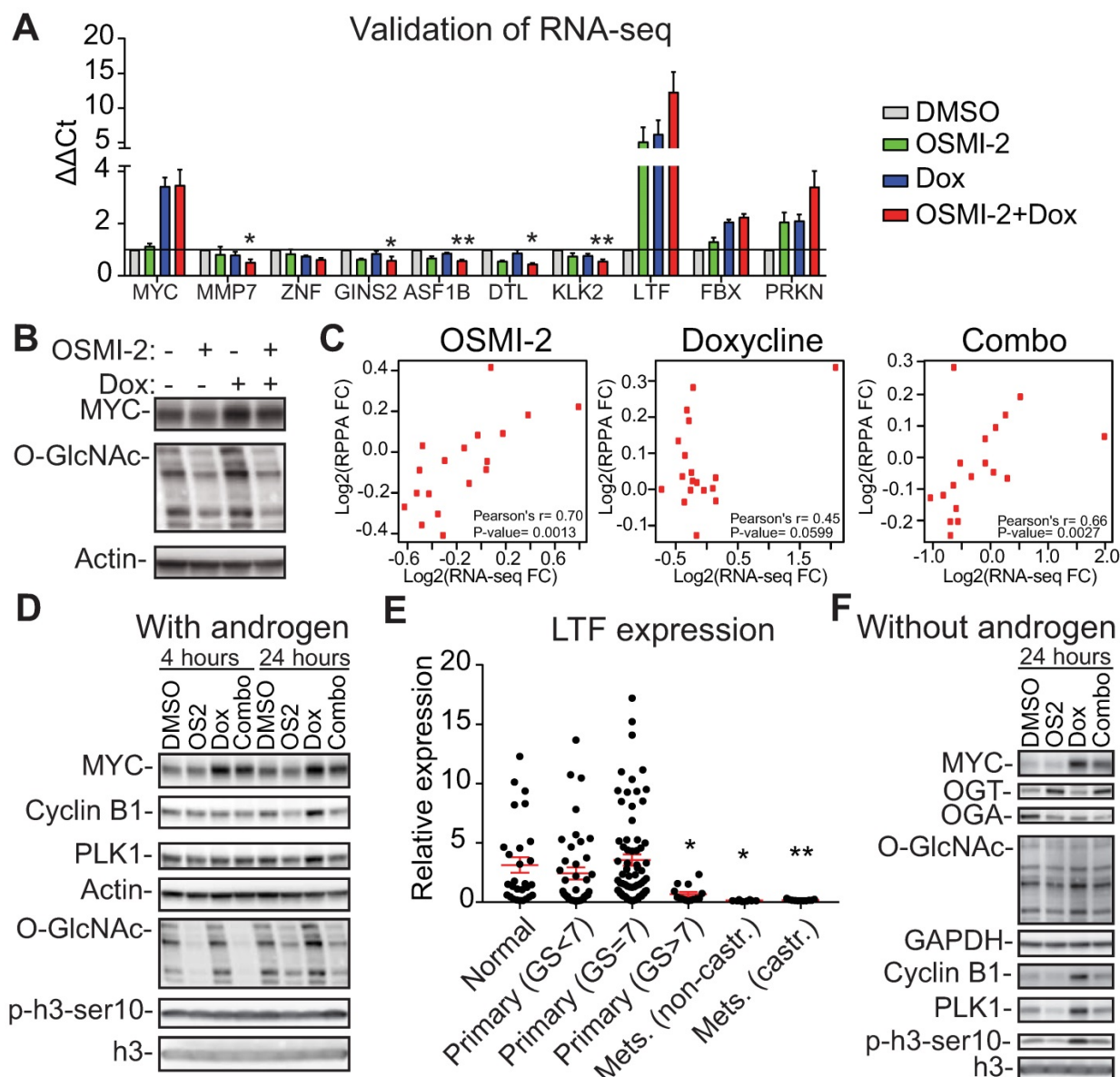
Figure 4. OGT affects MYC-dependent transcription. The expression of MYC was induced in the LNCaP-MYC cell line by addition of doxycycline (Dox). A ) Validation of the RNA-seq data using RT-qPCR. Treatment time is 24 hours and OSMI-2 dose 40µM. MMP7 , ZNF (=ZNF812P), GINS2 , ASF1B , DTL and KLK2 were down-regulated in the combination treatment with OSMI-2 and doxycycline (to induce MYC), while LTF , FBX (=FBXO32) and PRKN were up-regulated. Data shown is an average of three biological replicates with SEM. Student's t-test was used to evaluate statistical significance between Dox and Dox+OSMI-2 condition, * <0.05 and ** <0.01 . B ) Cells were treated with Dox and 40µM OSMI-2 for 24 hours and analyzed by western blotting. C ) Pearson correlation of mRNA and protein expression for the proteins that were induced by MYC-overexpression and antagonized by OSMI-2. D ) MYC-induced upregulation of PLK1 and Cyclin B1 is antagonized by OSMI-2 (OS2). Cells were treated as indicated and samples were analyzed using western blotting. E ) Expression of the LTF gene in prostate cancer patient samples. Data was downloaded from http://www.betastasis.com/prostate_cancer/taylor_et_al_2010 . The mean values with SEM are shown for each group. The significance of the data was evaluated using Student's t-test in comparison to normal samples, * <0.05 , ** <0.01 . F ) LNCaP-MYC cells were grown in the absence of androgens for 3 days, treated as indicated for an additional 24 hours, protein lysates were collected and western blot was used to detect the indicated proteins.
