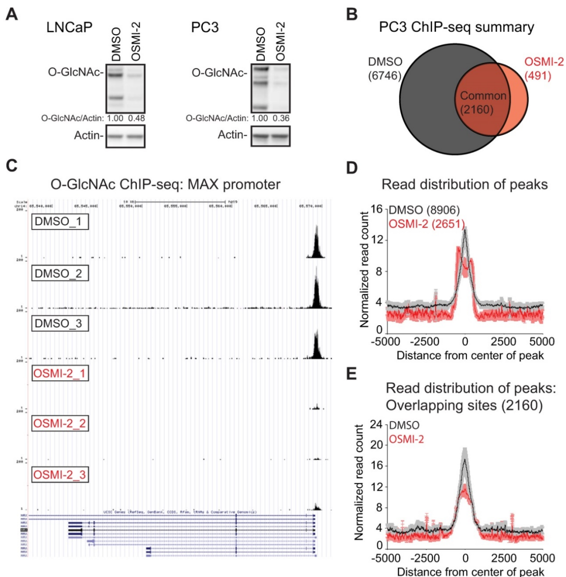
Figure 1. Global chromatin O-GlcNAc mark is sensitive to OGT inhibition. A) 40 \mu M OSMI-2 treatment rapidly decreases global O-GlcNAc levels as determined using western blot after 4 hours of treatment. B) Summary of the PC3 O-GlcNAc ChIP-seq data. Cells were treated for 4 hours with DMSO or 40 \mu M OSMI-2. The data shown represents overlap of three biological replicate samples for both DMSO and OSMI-2 treatments. C) OSMI-2 treatment decreases O-GlcNAc peak strength. University of California, Santa Cruz (UCSC) Genome Browser view of the Max gene promoter and three biological replicate O-GlcNAc ChIP-seq experiments. D) Distribution of O-GlcNAc ChIP-seq reads within \pm 5kb of O-GlcNAcylated regions within either DMSO or OSMI-2 conditions. Data shown is an average of three biological replicates with SEM. E) Distribution of O-GlcNAc ChIP-seq reads within \pm 5kb of O-GlcNAcylated regions overlapping within DMSO and OSMI-2 conditions. Data shown is an average of three biological replicates with SEM.
