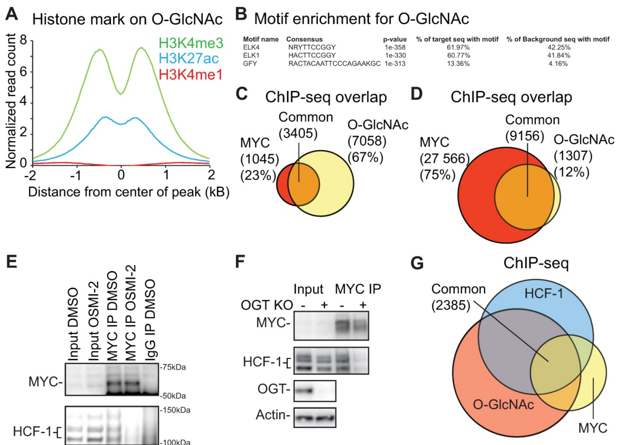
Figure 3. Identification of transcription factors that bind to O-GlcNAc marked chromatin. A) Distribution of differently modified histone 3 reads within ±2kb of O-GlcNAc peak. B) The top 3 motifs enriched for the O-GlcNAc ChIP-seq data showing similarity with known previously identified transcription factor motifs from published datasets. C) O-GlcNAc ChIP-seq consensus overlap with MYC ChIP-seq data reported in this study. D) O-GlcNAc ChIP-seq consensus overlap with MYC ChIP-exo dataset reported previously (GSE73994). E) OSMI-2 disrupts interaction between MYC and HCF-1. Immunoprecipitation (IP) of MYC. IgG denotes negative control. MYC was overexpressed by addition of doxycycline using the LNCaP-MYC cell line for 4 hours either in the presence or absence of 40µM OSMI-2. Experiment was repeated four times. F) Knockout of OGT disrupts the interaction between MYC and HCF-1. Experiment was performed in a mouse embryonic fibroblast cell line that has been genetically engineered to enable removal of OGT gene by addition of 0.5µM Tamoxifen (Tam). After two days of DMSO- or Tam-treatments, cell lysates were prepared and used for immunoprecipitation. Data shown is representative of two biological replicates. G) Overlap of O-GlcNAc (this study), MYC (this study) and HCF-1 (ENCSR000ECH) ChIP-seq data.
