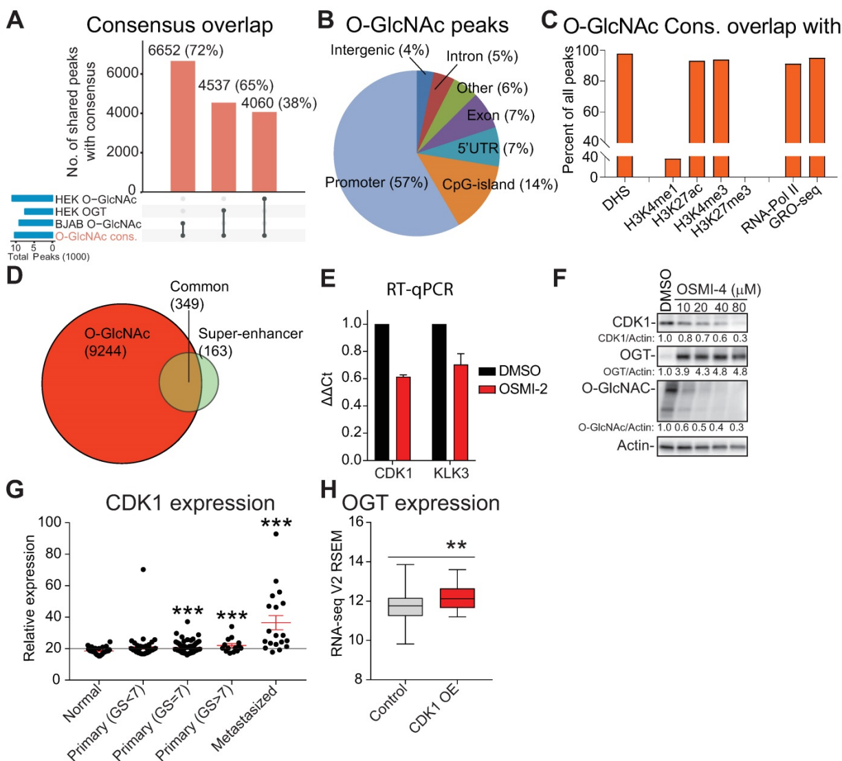
Figure 2. O-GlcNAc chromatin mark overlaps with active promoters and super-enhancers. A ) UpSet plot shows the overlap of O-GlcNAc consensus peak-set (10,463) with previously reported OGT and O-GlcNAc ChIP-seq datasets [BJAB O-GlcNAc [GSM2295951], HEK OGT [GSE36620], and HEK O-GlcNAc [GSE36620]]. B ) Peak distribution of O-GlcNAc ChIP-seq data reported here with respect to known genomic elements. C ) O-GlcNAc consensus overlap with previously published datasets. Accession numbers to published datasets: DNase I hypersensitive site (DHS): GSM816637, H3K4me1: GSE73994, H3K27ac: GSE73994, H3K4me3: GSE73994, H3K27me3: GSE73994, RNA-Pol II: GSE28126 and Global Run-On Sequencing (GRO-seq); retrieved from Wang et al. , 2011 and analyzed according to Chae et al. , 2015 [73, 74]. D ) Overlap of LNCaP O-GlcNAc ChIP-seq marked genes with LNCaP super-enhancers as reported previously [47]. E ) The effect of 40 μM OSMI-2 (24 hours) on CDK1 and KLK3 mRNA expression. The data shown is an average of three biological replicates with SEM. F ) The effect of OSMI-4 (24 hours) on CDK1 expression at the protein level. Densitometry was used to determine the intensity of the indicated proteins. G ) Expression of the CDK1 gene in prostate cancer patient samples. Data was downloaded from http://www.betastasis.com/prostate_cancer/taylor_et_al_2010 . The mean values with SEM are shown for each group. The significance of the data was evaluated using Student's t-test in comparison to normal samples, ***<0.001. H ) Expression of OGT in prostate cancer tumor samples that overexpress CDK1 (n=19) and the rest (n=479). The figure was generated using data available through cBioPortal [75, 76].
